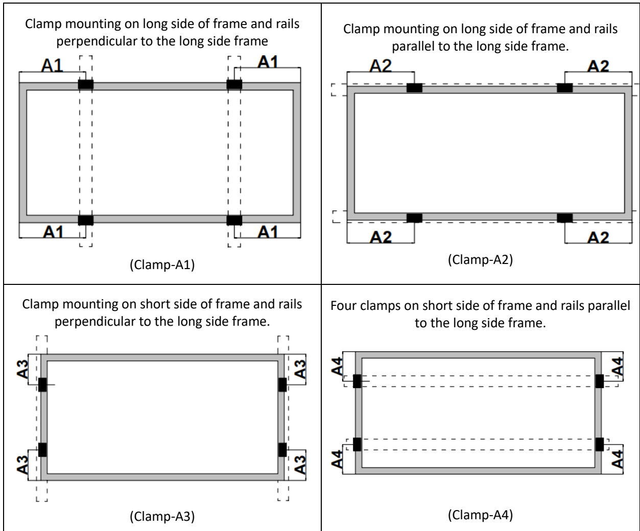
Approved Clamp mounting
